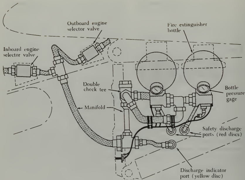
FIGURE 9-13. Dual container installation and fittings.
